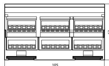
on a 35 mm top-hat rail (in accordance with DIN EN 60715 TH35)
