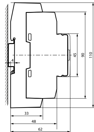
on a 35 mm top-hat rail (in accordance with DIN EN 60715 TH35)
