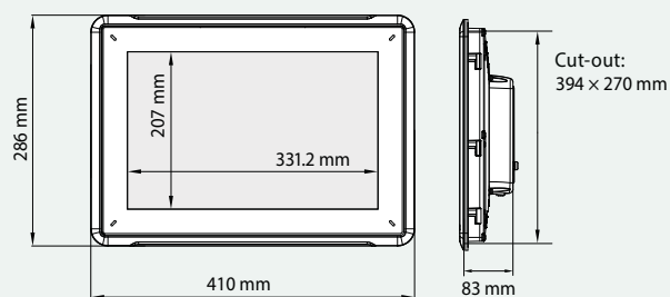
15" Panel PC PCD7.D5150WTC010
