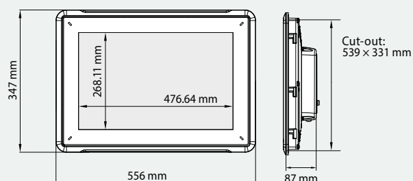
21" Panel PC PCD7.D6210WTI010
